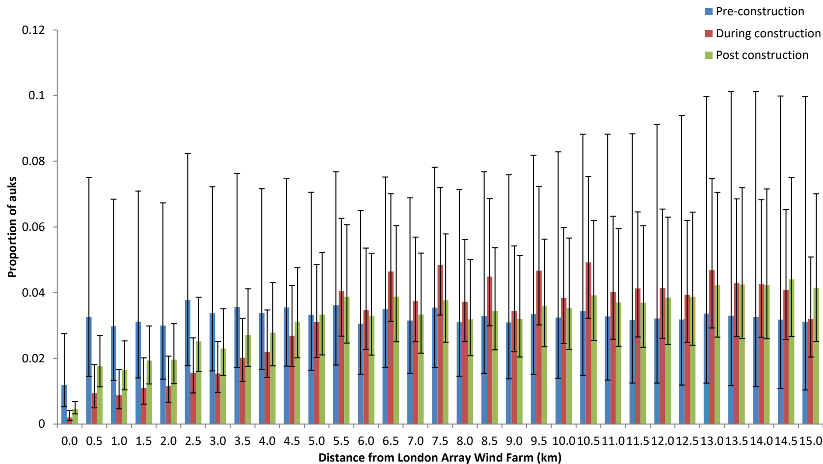
Figure 43 Proportion of auks ( \pm 95% confidence intervals generated during the modelling process) by distance to the London Array Wind Farm.
