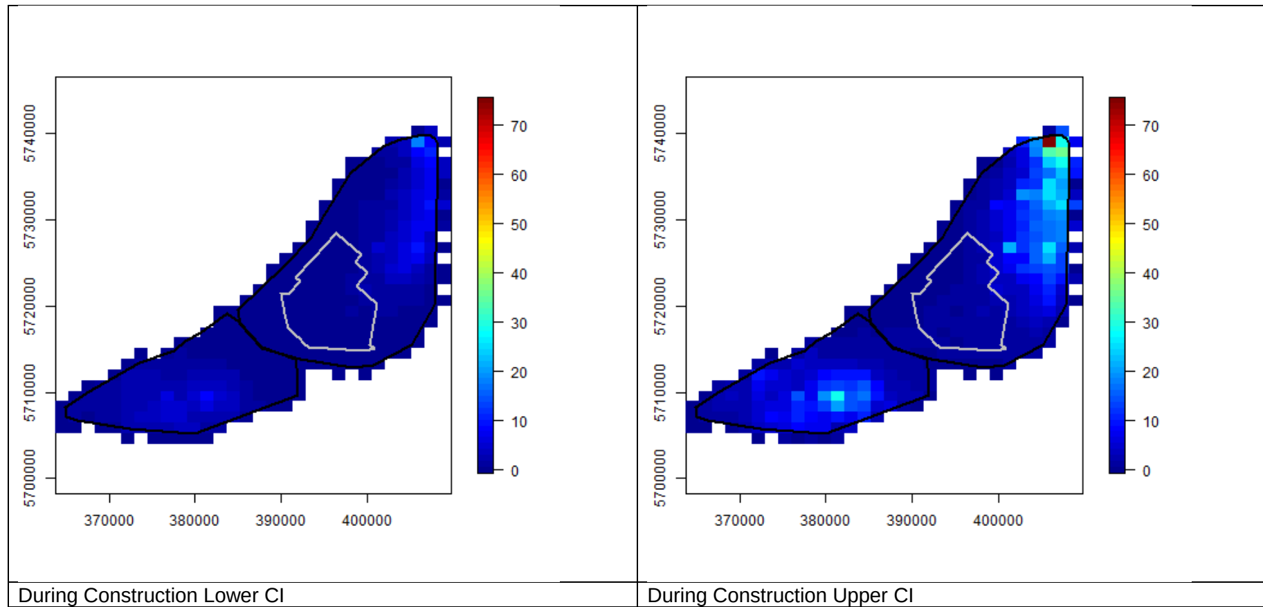
Figure 25 During construction diver density (birds \text{km}^{-2} ) lower and upper confidence limits.
